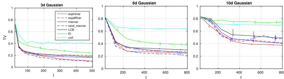
Figure 6: Median of the average marginal TVs between the estimated ABC posterior and the corresponding true posterior over 100 experiments in the 3d, 6d and 10d Gaussian toy simulation model.
