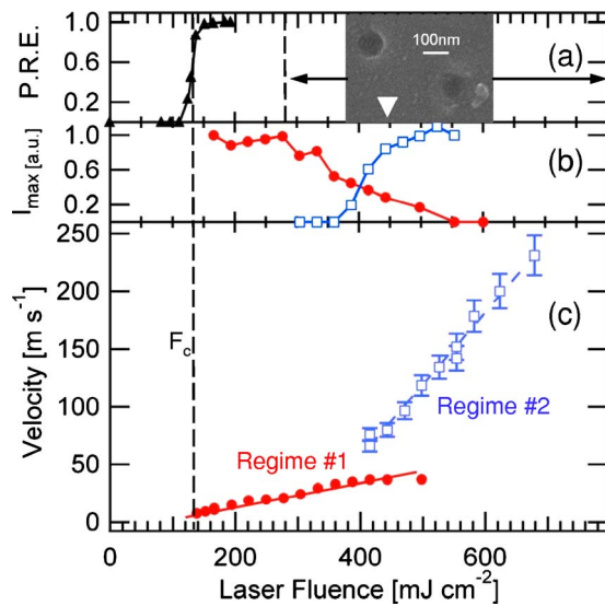
FIG. 2. (Color online) (a) Particle Removal Efficiency (PRE), (b) maximum scattering intensity I_{max} , and (c) particle velocity corresponding to each ejected cloud as a function of the laser fluence F_{las} . The scattered intensity for the slow (fast) component was measured for a time delay t set to 10 \mu s (20 \mu s). The embedded SEM image shows the ablated craters observed for F_{las} \approx 430 mJ cm -2 .
