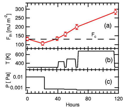
FIG. 3. (Color online) (a) Increase of the particle removal fluence threshold F_{th} over time when water vapor progressively desorbs from surfaces. (b) The sample holder in the vacuum chamber is backside equipped with a halogen lamp to perform successive baking steps under (c) a decreasing atmosphere pressure.
