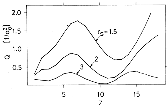
FIG. 3. Electron transport cross section at Fermi level defined via Eq. (4) for atoms in an electron gas with the density parameter r_s = 1.5, 2 , and 3 . For r_s = 2 , see also Fig. 4. The dashed part of the r_s = 3 curve corresponds to atoms for which we did not find fully converged solutions.
