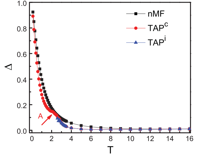
FIG. 2. (Color online) The reconstruction error \Delta with temperature T for both nMF and TAP approximation. The other parameter values: N = 20 , data length L = 20 \times 10^6 , external field \theta = 0 , asymmetric degree k = 1 . Black squares, nMF; red circles, cubic equation method for TAP; blue triangles, iterative method for TAP. Each data point is averaged on 10 realizations.
